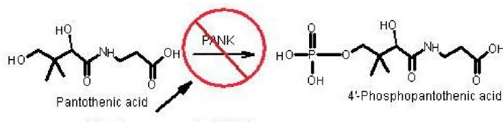
Missing enzyme in PKAN
